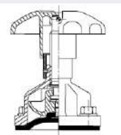
Cast iron bonnet with rising plastic handwheel DN15 - DN50 1/2" - 2"
