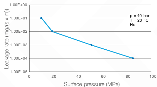
Tightness performance
